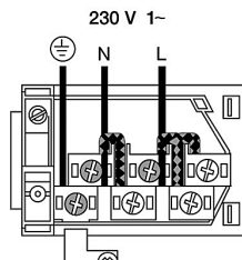
3 x 4mm 2
