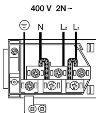
4 x 2,5mm 2
