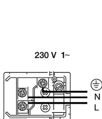
3 x 1,5mm 2
